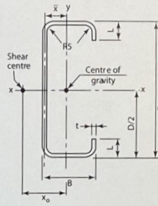
C-Purlin
