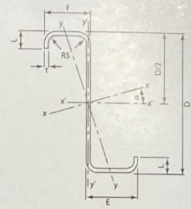
Z-Purlin
